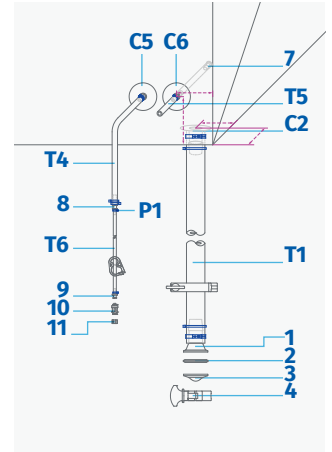
DETAIL B
